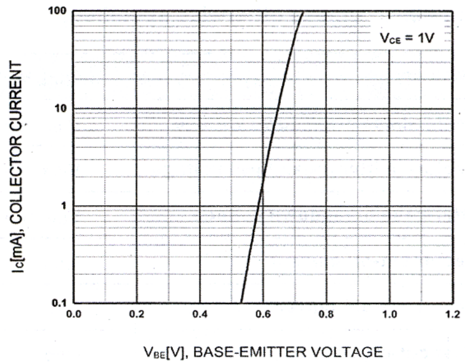
Base-Emitter On Voltage
