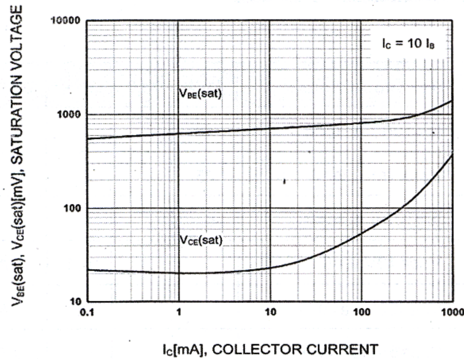
Base-Emitter Saturation Voltage Collector-Emmitter Saturation Voltage
