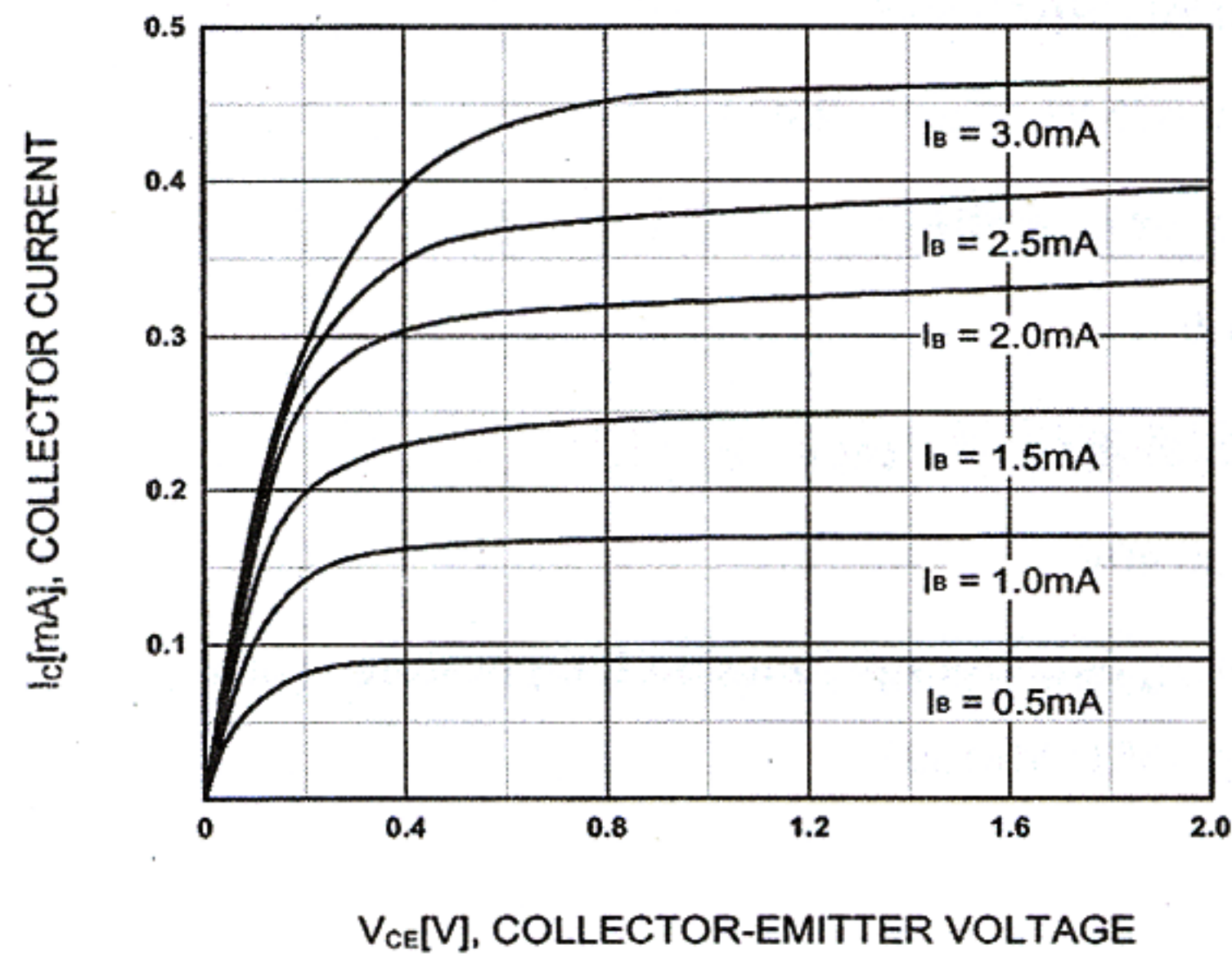
Static Characteristic
