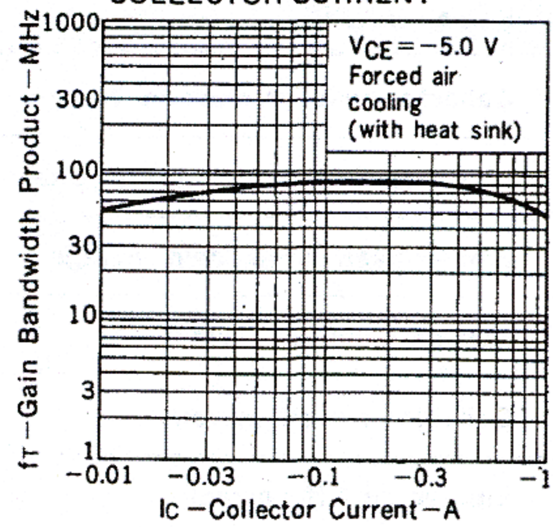
GAIN BANDWIDTH PRODUCT vs. COLLECTOR CURRENT
