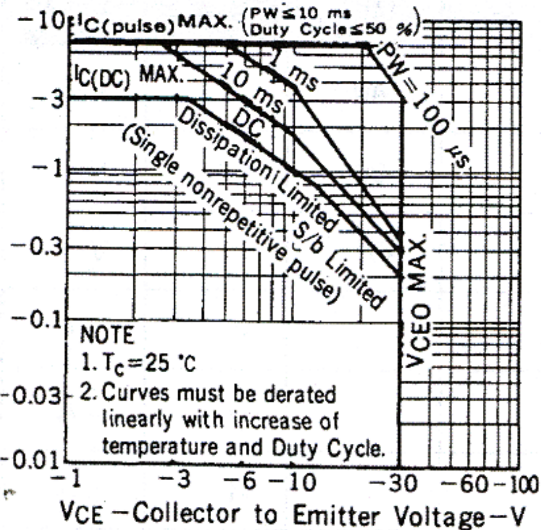
SAFE OPERATING AREAS
